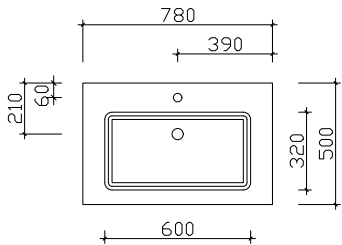
Breite 780 mm BME015F78002
